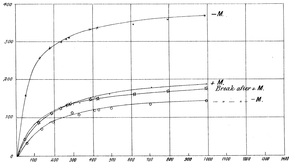
Temperature 100° Cent. M & B with 21 lbs. on.
