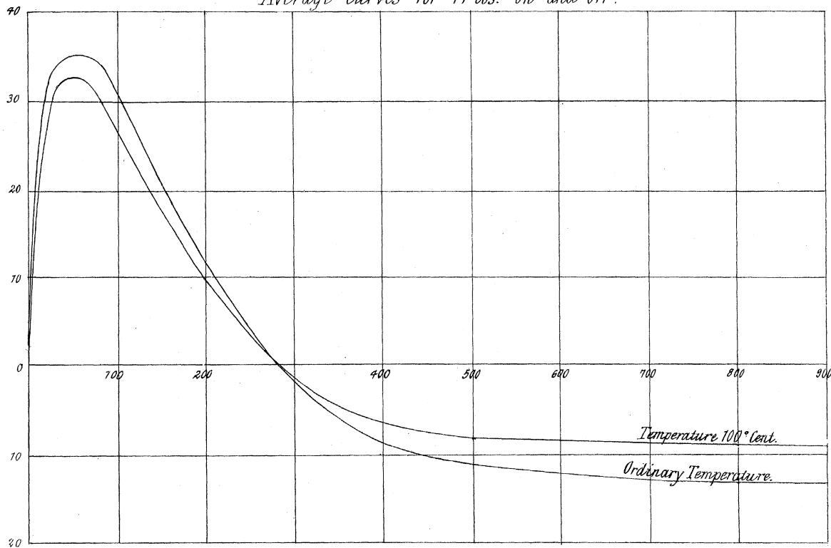
Average curves for 14 lbs. "on and off."
